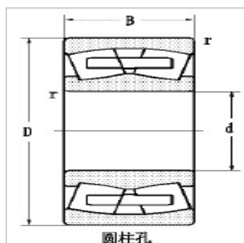
圆柱孔
